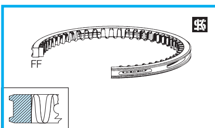
FF Formflex-Ring
