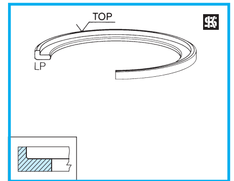
LP L-Profilring
